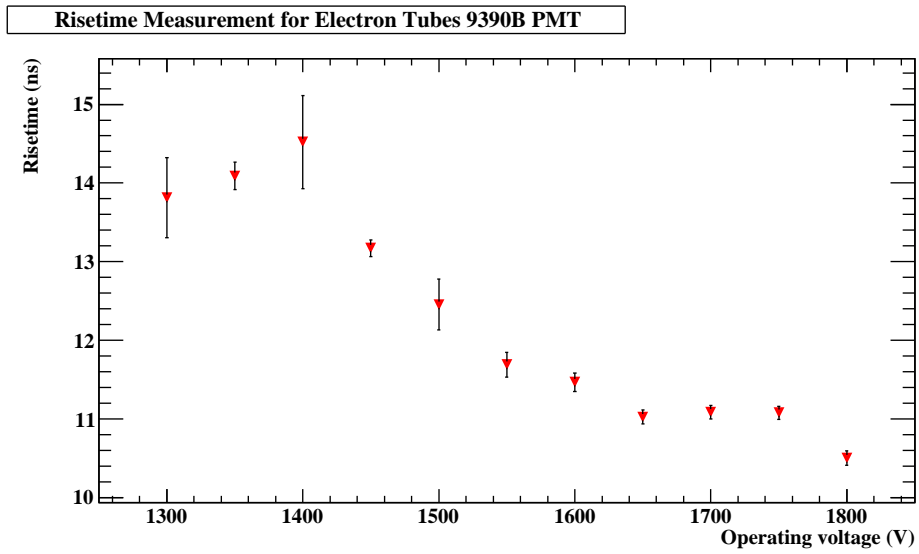
Figure 5.34: Risetime measurement for the Electron Tubes 9390B PMT calculated from the spectra collected using the TPHC.
