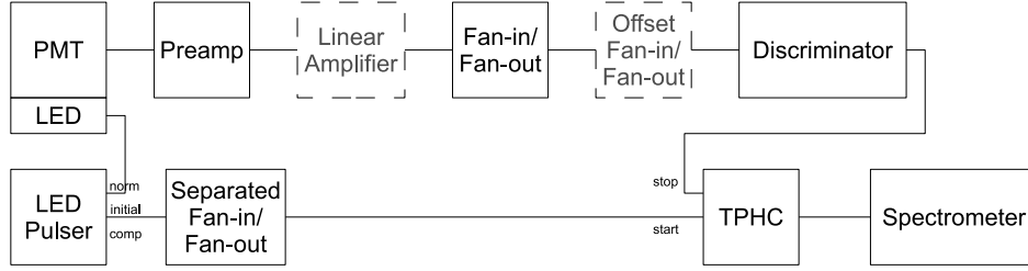
Figure 5.29: A simplified flowchart of the DAQ setup for measuring the time resolution of the PMTs using a TPHC.
