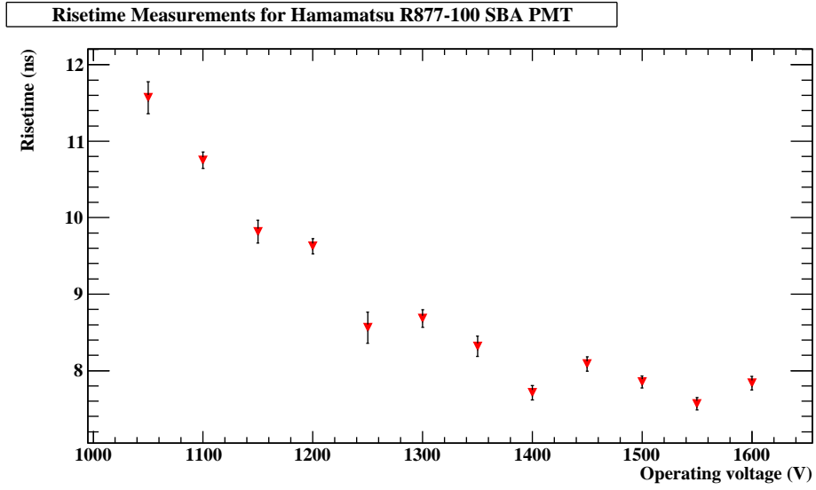
Figure 5.33: Risetime measurement for the Hamamatsu R877-100 SBA PMT calculated from the spectra collected using the TPHC.
