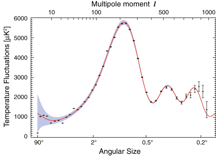
Figure 1.4: The power spectrum of the CMB from five years of WMAP data. This figure compares the angular size of the bright spots on the CMB map (Figure 1.3) to the magnitude of their temperature fluctuations (using a calculated quantity that includes the multipole moments). Each peak represents a different source of the fluctuations. (NASA [31]).
