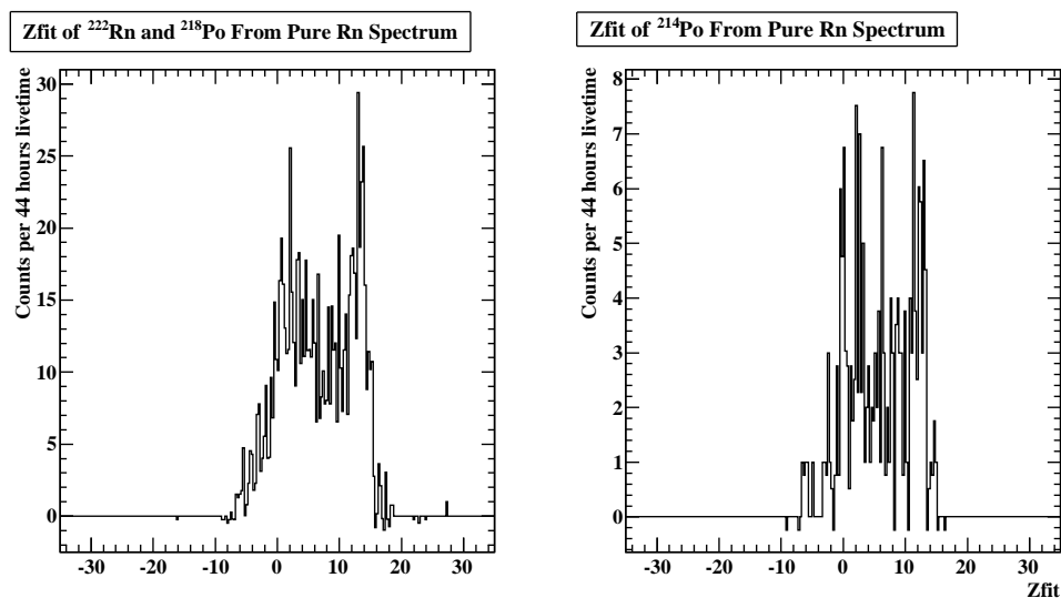
Figure 3.9: The Zfit distribution of events for the two peaks in Figure 3.5. The peak due to ^{214}\text{Po} and that due to ^{222}\text{Rn} and ^{218}\text{Po} both show a concentration of events in the argon bulk.
