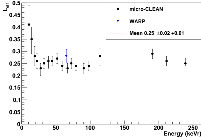
Figure 2.5: \mathcal{L}_{\text{eff}} as a function of recoil energy. The cause of the upturn below 20 keV r is not known, and the red line is the weighted mean for events above 20 keV r [114]. Included is a measurement made by the WArP collaboration [117].
